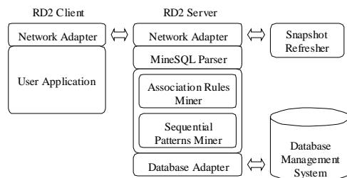
Fig. 1. RD2 Architecture
